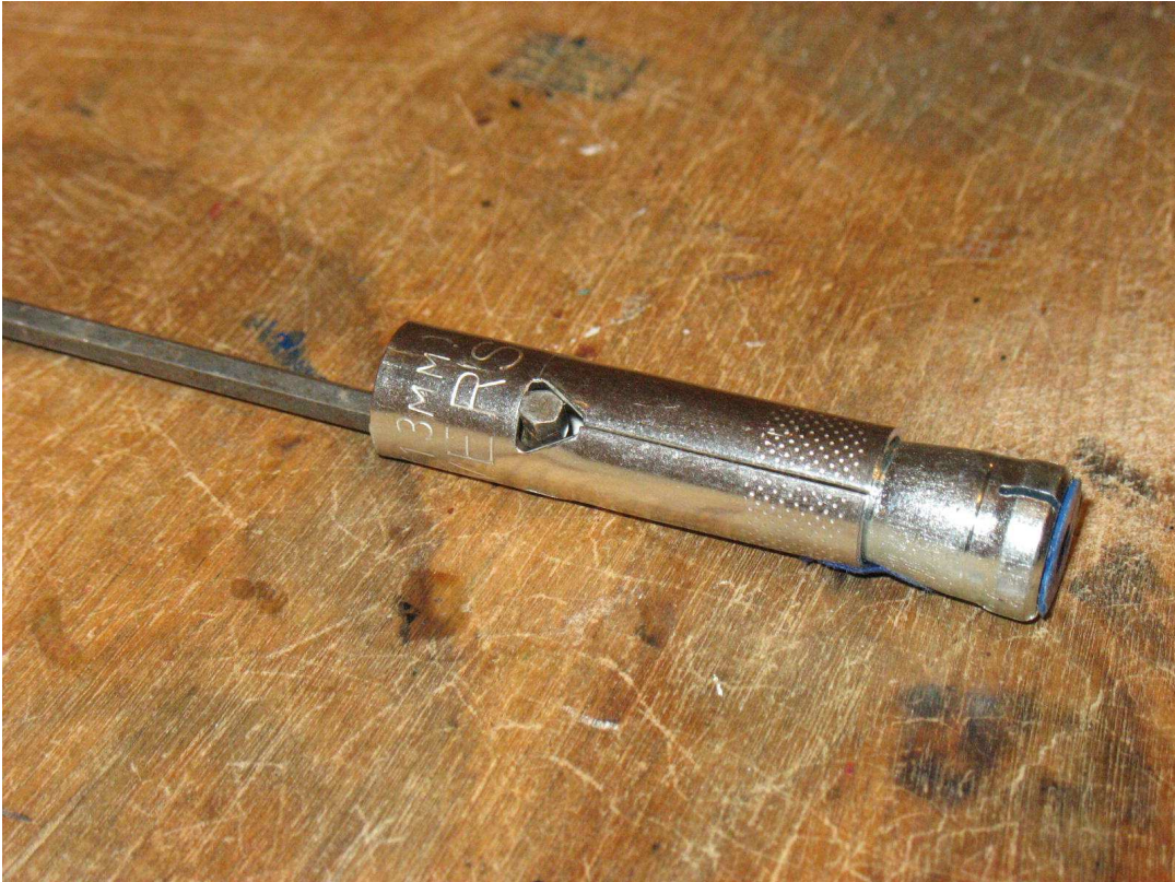
T-hex handle engaged into triangular hole of expansion sleeve
